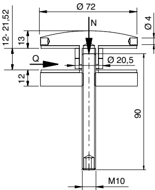
Ø 72 mm, erhaben | Ø 72, raised
