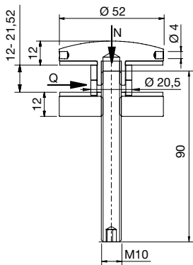
Ø 52 mm, erhaben | Ø 52, raised
